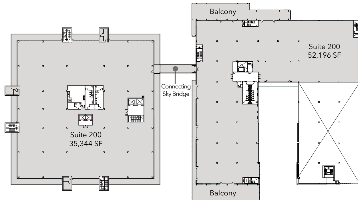
As-Built 2nd Floor (Press)
